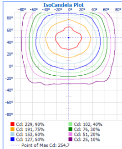
Isocandela Plot
