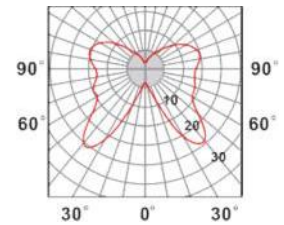
Light distribution
