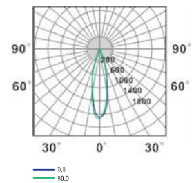
Light distribution
