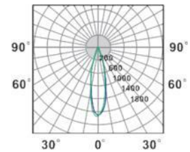
Light distribution
